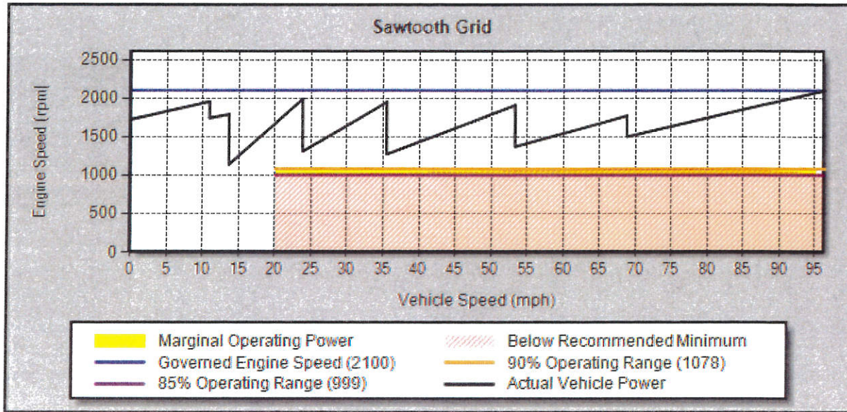
Sawtooth Details
